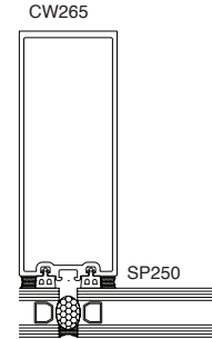
③ SILL
