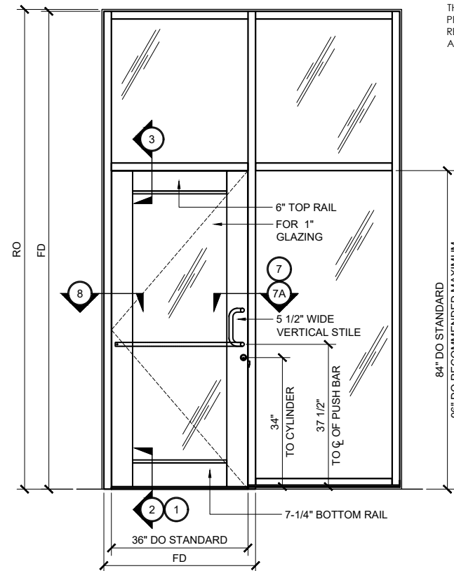
WIDE STILE SERIES 550AT DOOR TYP. ELEVATION (SINGLE DOOR @ TRANSOM FRAME) 3/4" = 1'-0"
