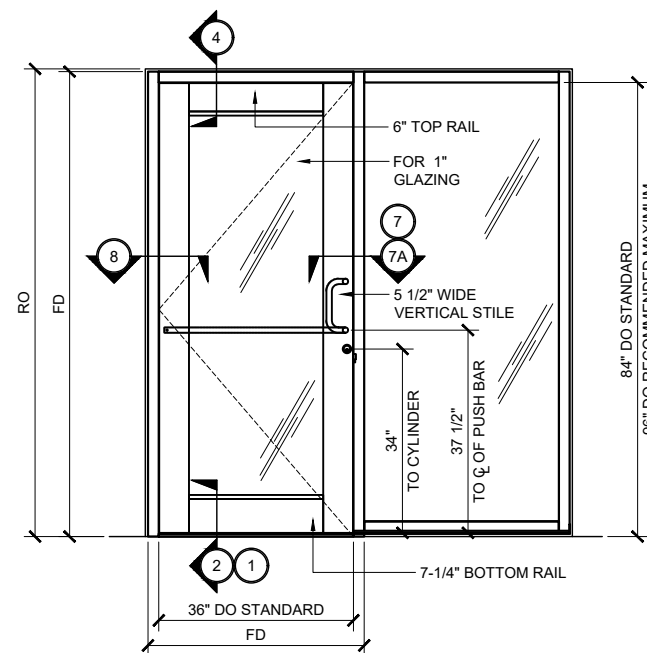
WIDE STILE SERIES 550AT DOOR TYP. ELEVATION (SINGLE DOOR @ UP / OVER FRAME WITH SIDELITE) 3/4" = 1'-0"
