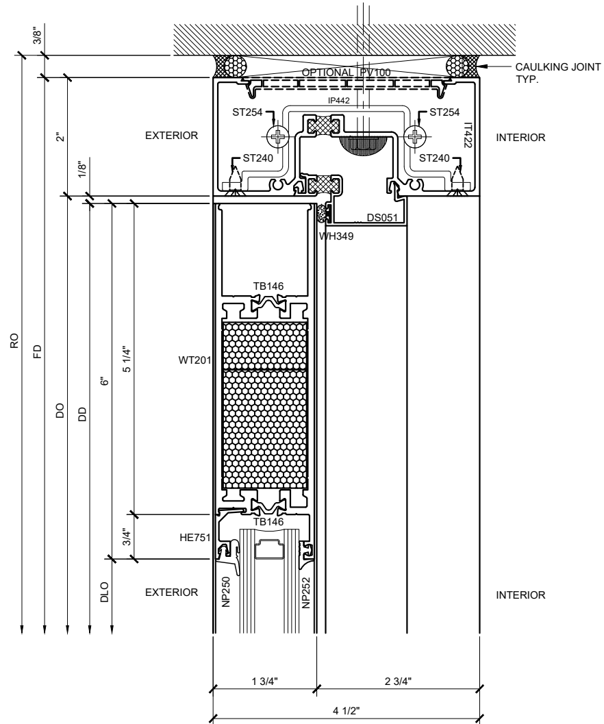
SECTION DETAIL @ DOOR HEAD 4 SCALE: FULL SIZE
