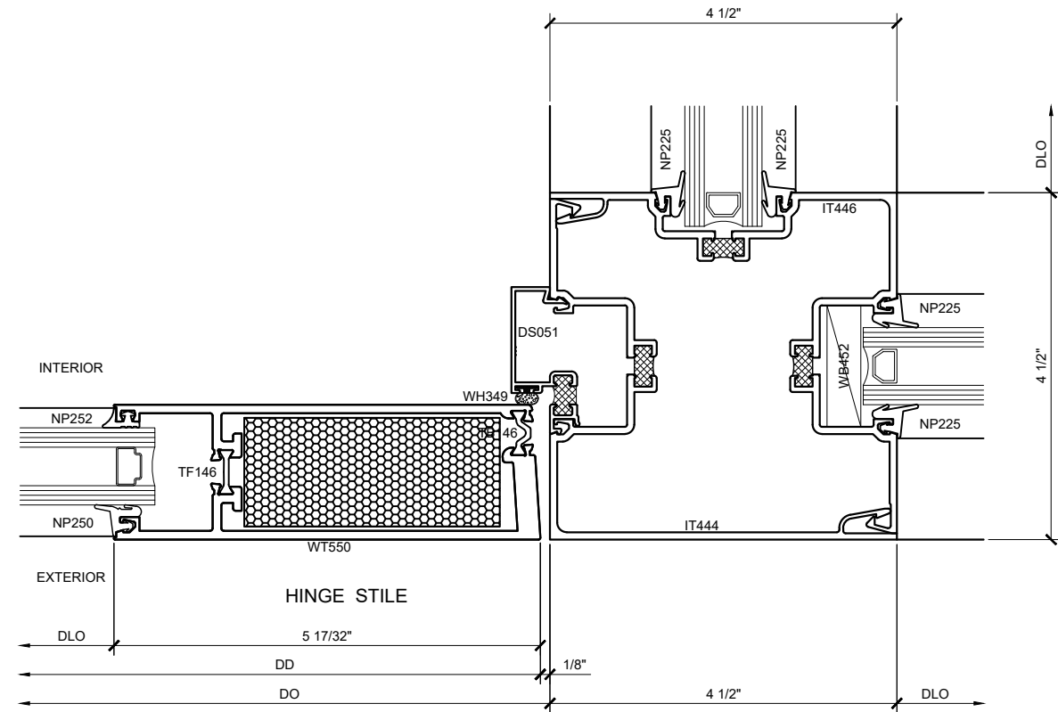
SECTION DETAIL AT WIDE HINGE STYLE "T" VERTICAL (13) SCALE: FULL SIZE
