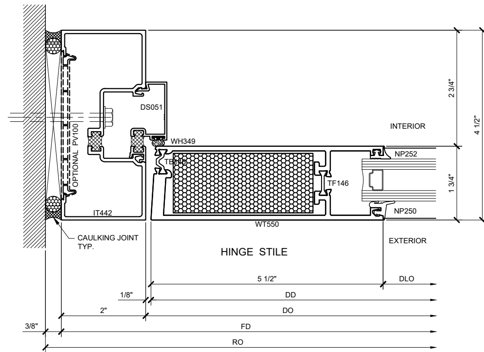
SECTION DETAIL @ DOOR HINGE JAMB
