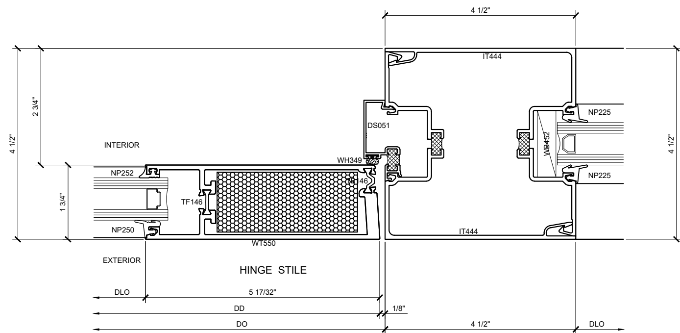
SECTION DETAIL AT WIDE HINGE STYLE INTERMEDIATE VERTICAL (14) SCALE: FULL SIZE
