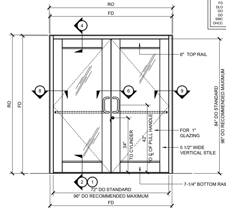
WIDE STILE SERIES 550AT DOOR TYP. ELEVATION (DOUBLE DOOR @ UP / OVER FRAME) 3/4" = 1'-0"
