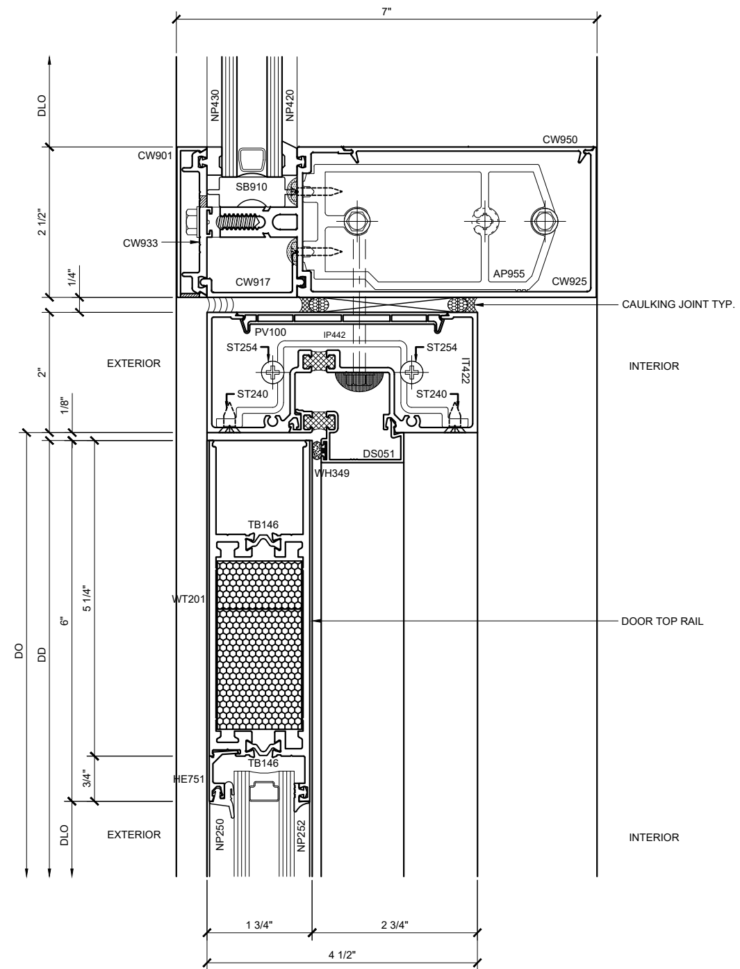
SECTION DETAIL @ DOOR HEAD (4A) SCALE: FULL SIZE
