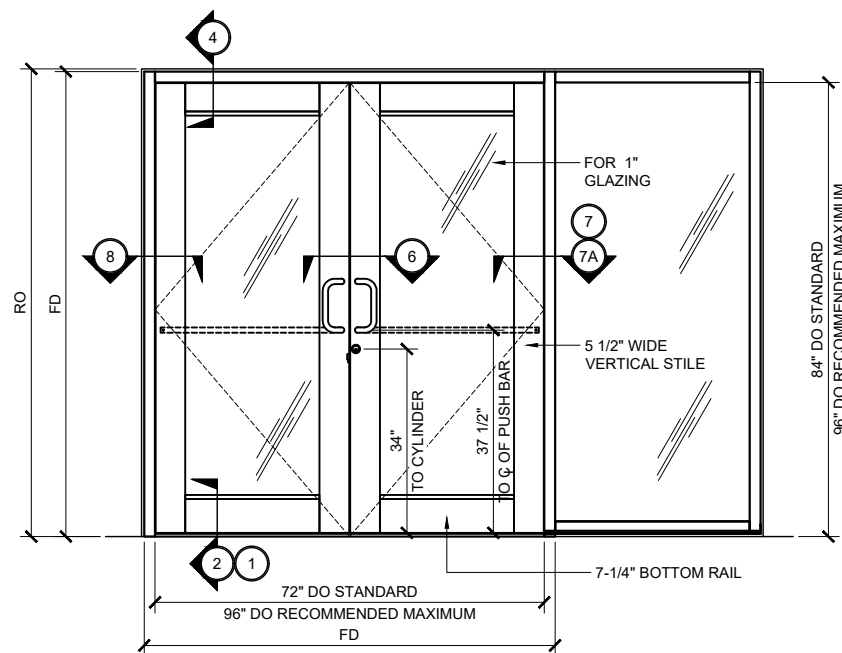
WIDE STILE SERIES 550AT DOOR TYP. ELEVATION (DOUBLE DOOR @ UP / OVER FRAME WITH SIDELITE) 3/4" = 1'-0"
