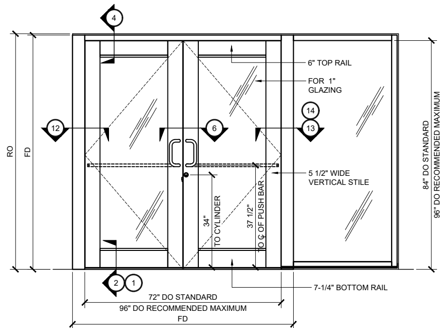
WIDE STILE SERIES 550AT DOOR TYP. ELEVATION (DOUBLE DOOR @ UP / OVER FRAME WITH SIDELITE) 3/4" = 1'-0"
