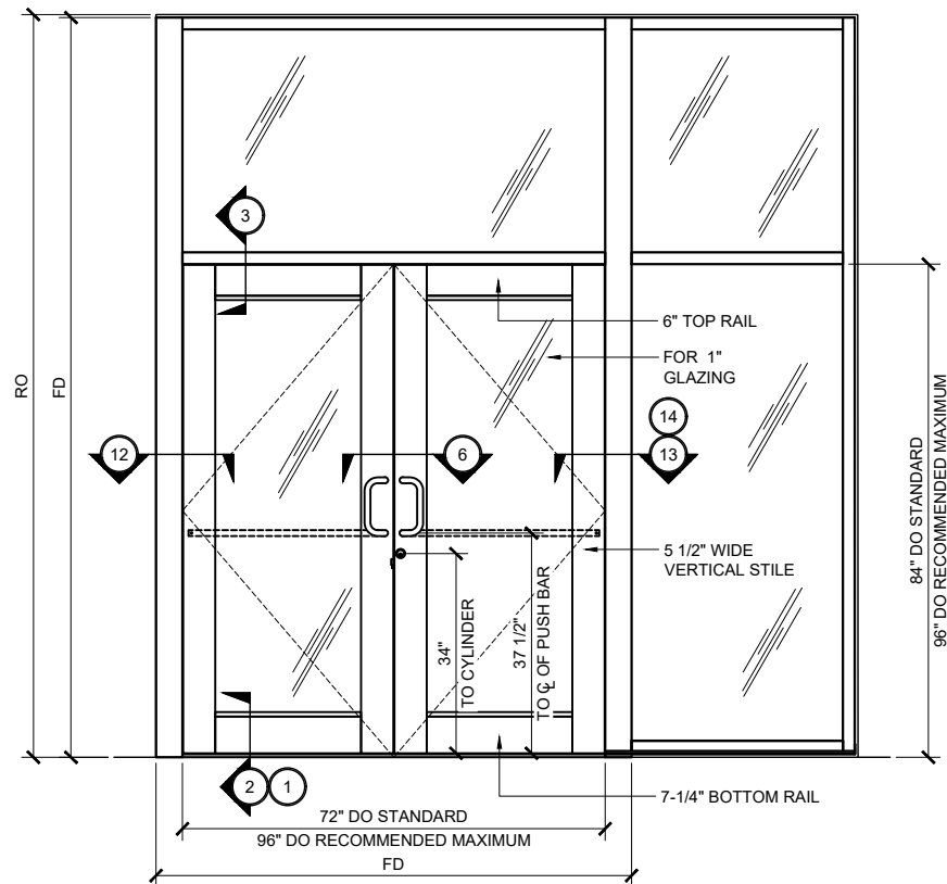
WIDE STILE SERIES 550AT DOOR TYP. ELEVATION (DOUBLE DOOR @ TRANSOM FRAME ) 3/4" = 1'-0"
