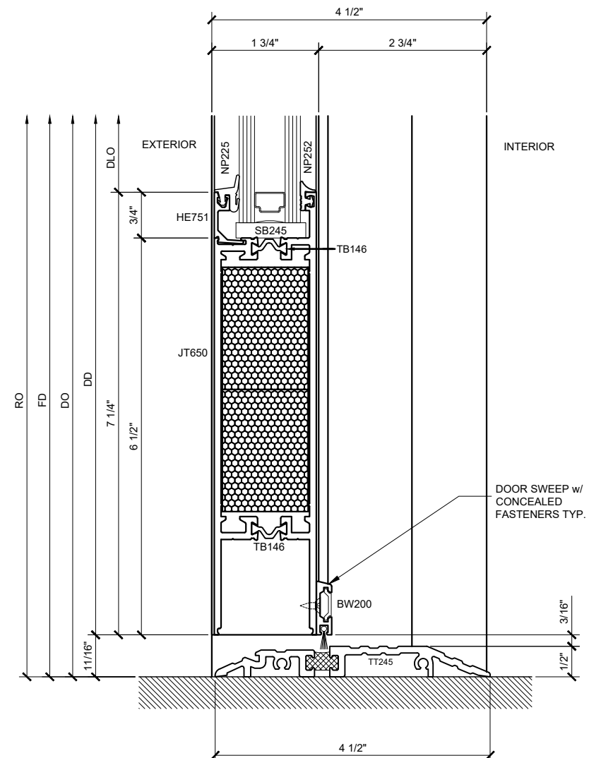
SECTION DETAIL @ 7" DOOR SILL ② SCALE: FULL SIZE
