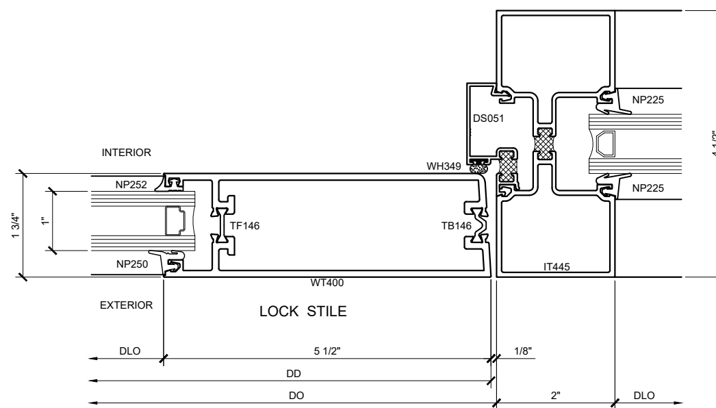
SECTION DETAIL @ DOOR JAMB (7A) SCALE: FULL SIZE
