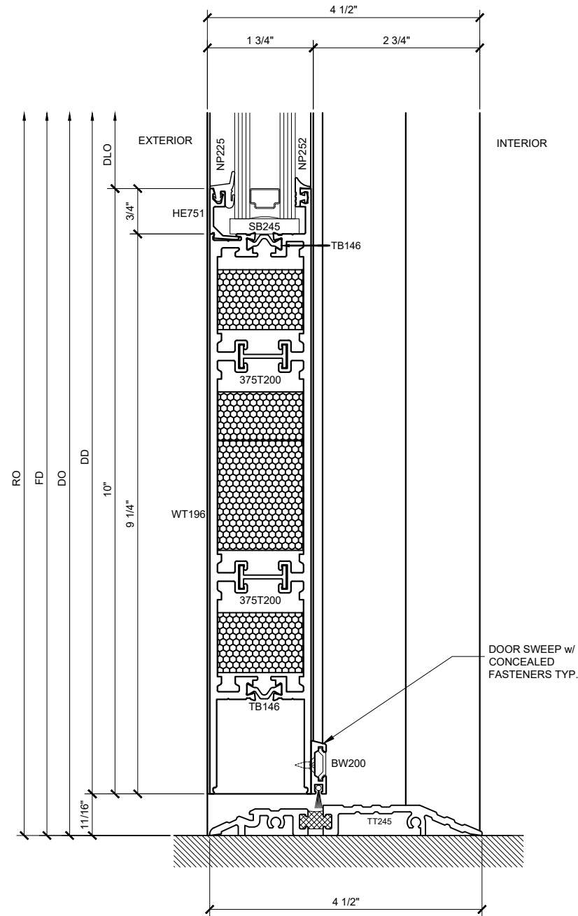
SECTION DETAIL @ 10" DOOR SILL ① SCALE: FULL SIZE
