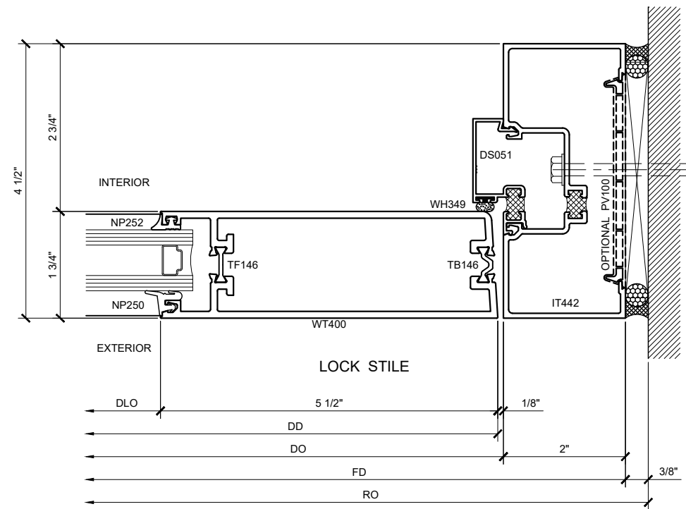
SECTION DETAIL @ DOOR JAMB
