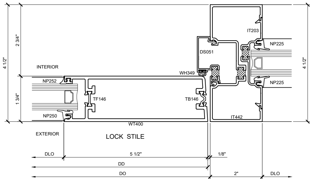
SECTION DETAIL @ DOOR JAMB (7) SCALE: FULL SIZE
