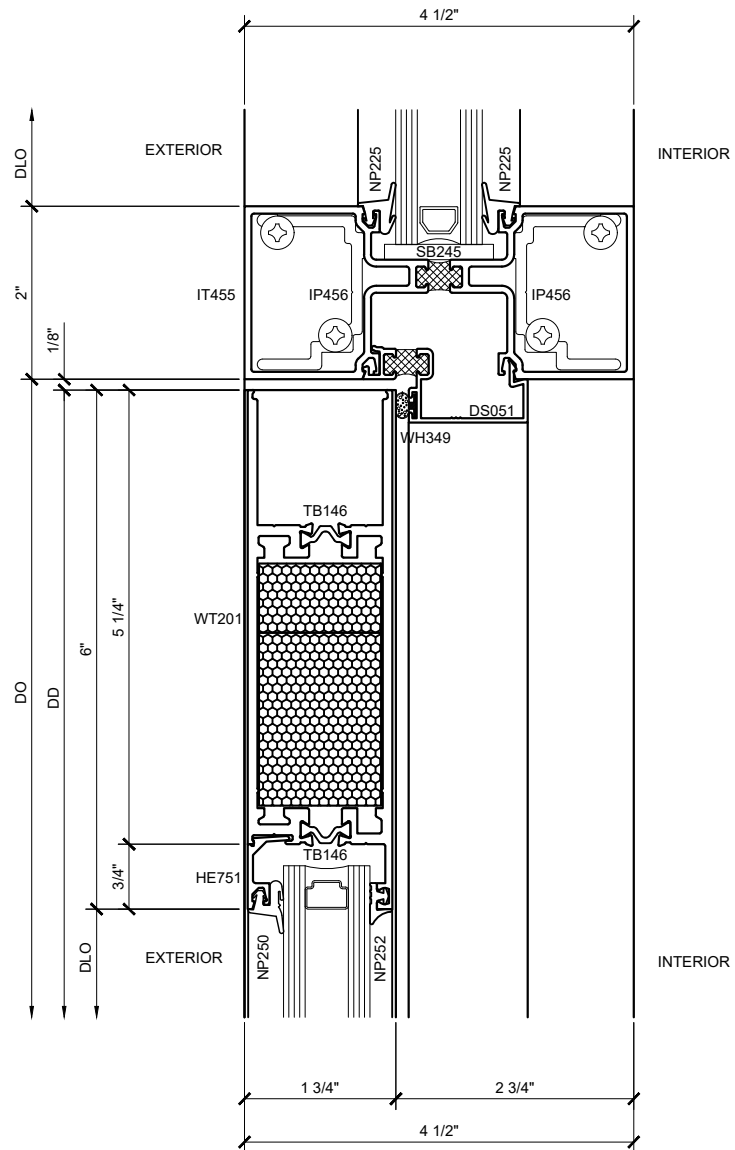
SECTION DETAIL @ TRANSOM 3 SCALE: FULL SIZE
