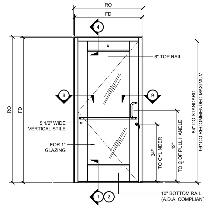
WIDE STILE SERIES 550AT DOOR TYP. ELEVATION (SINGLE DOOR @ UP / OVER FRAME) (SHOWN W/ 10" BOTTOM RAIL) 3/4" = 1'-0"
