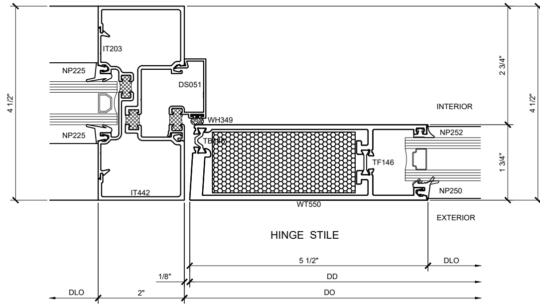
SECTION DETAIL @ DOOR HINGE JAMB (5) SCALE: FULL SIZE
