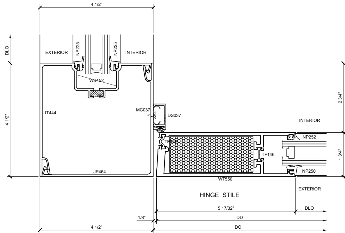
SECTION DETAIL AT WIDE HINGE STYLE CORNER VERTICAL (12) SCALE: FULL SIZE
