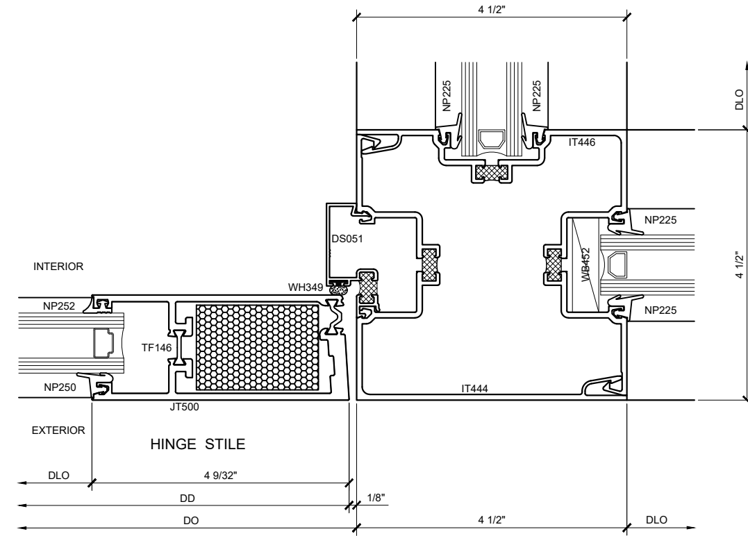
SECTION DETAIL AT WIDE HINGE STYLE "T" VERTICAL (13) SCALE: FULL SIZE
