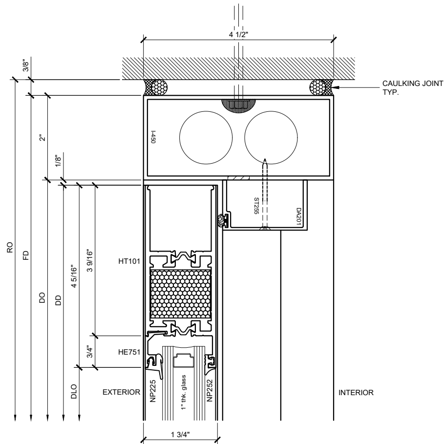
SECTION DETAIL @ DOOR HEAD w/ OHCC ⑤ SCALE: FULL SIZE
