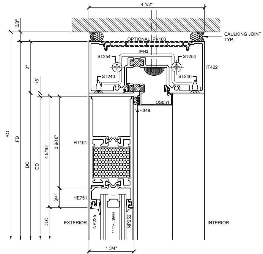
SECTION DETAIL @ DOOR HEAD ⑥ SCALE: FULL SIZE
