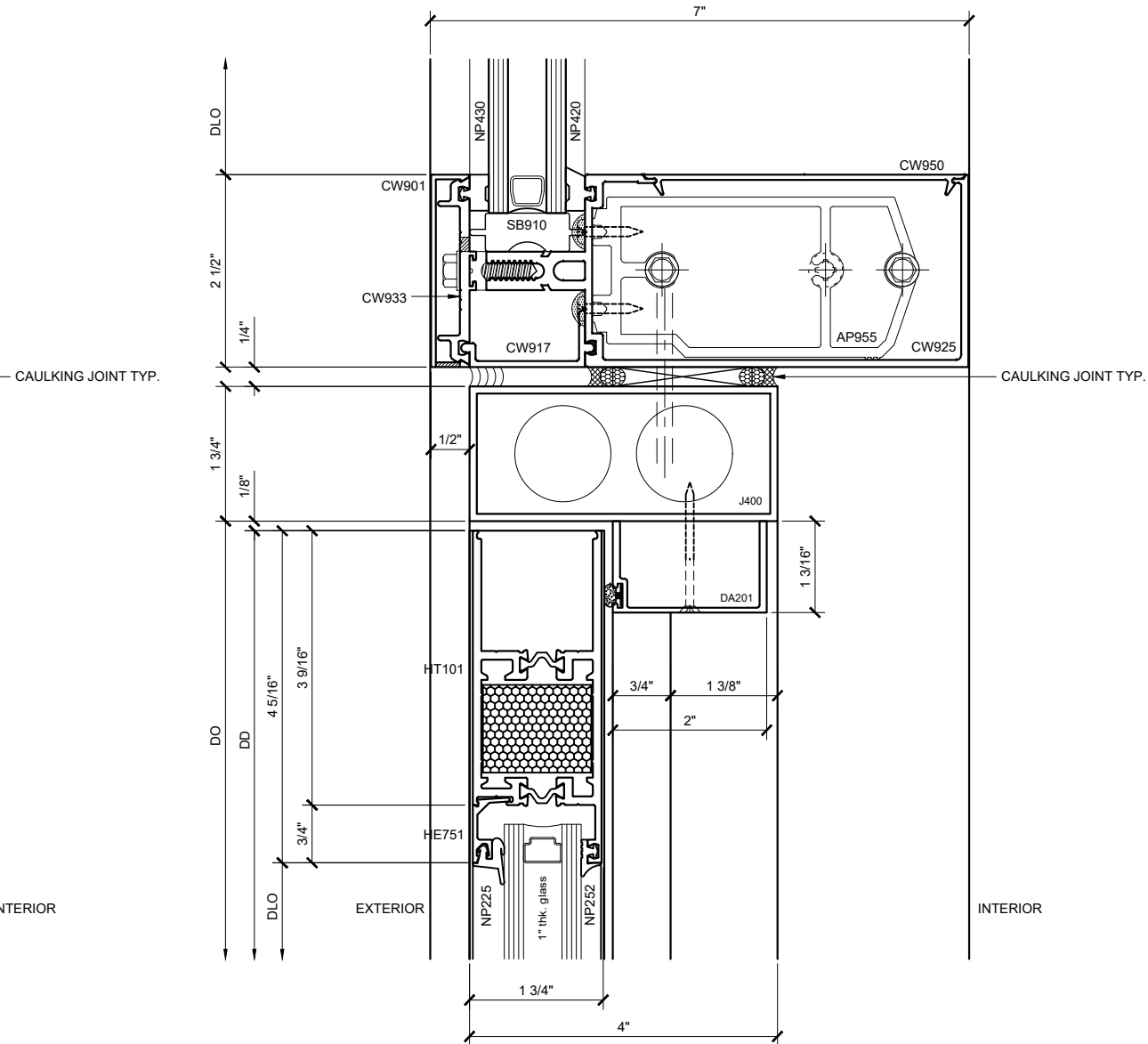
SECTION DETAIL @ DOOR HEAD w/ OHCC 19 SCALE: FULL SIZE
