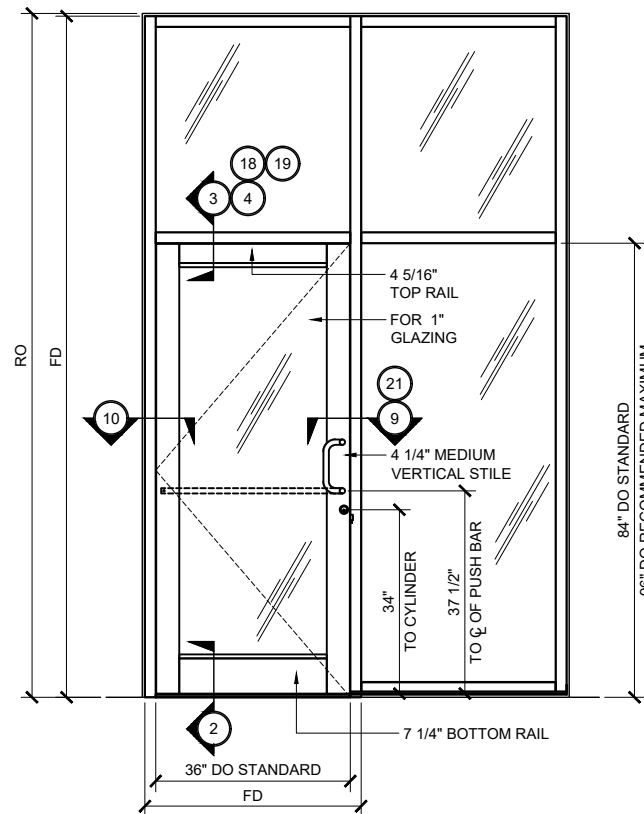
MEDIUM STILE SERIES 400AT DOOR TYP. ELEVATION (SINGLE DOOR @ TRANSOM FRAME) 3/4" = 1'-0"
