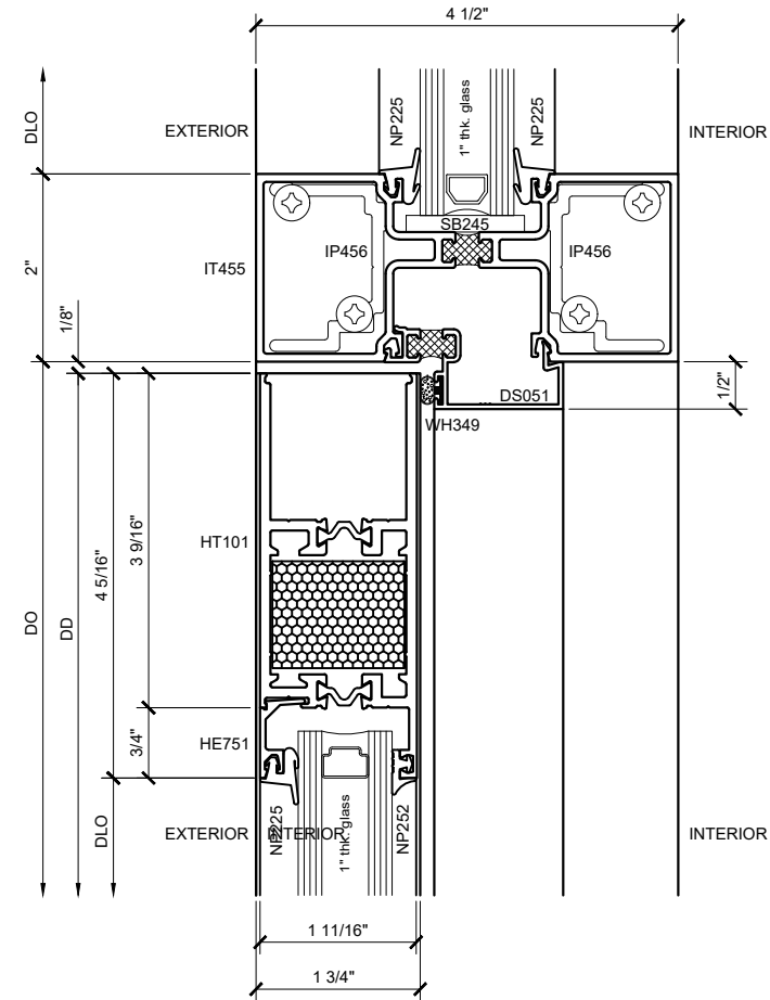
SECTION DETAIL @ DOOR HEAD ④ SCALE: FULL SIZE
