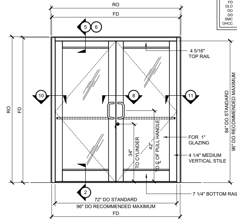
MEDIUM STILE SERIES 400AT DOOR TYP. ELEVATION (DOUBLE DOOR @ UP / OVER FRAME) 3/4" = 1'-0"
