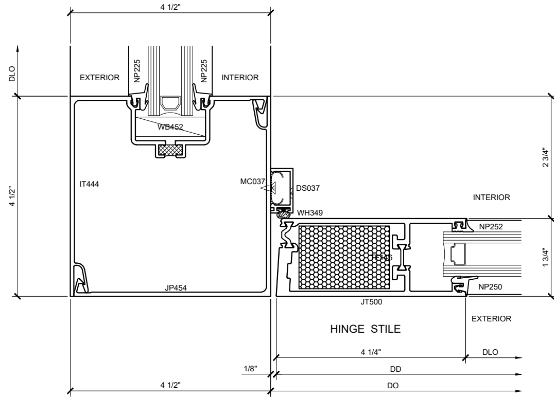
SECTION DETAIL AT WIDE HINGE STYLE CORNER VERTICAL (12) SCALE: FULL SIZE
