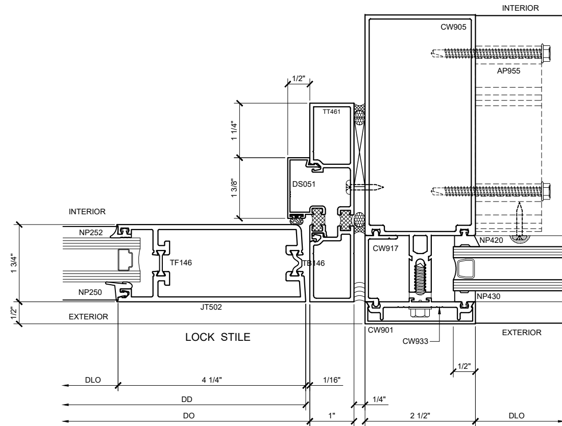
SECTION DETAIL @ DOOR JAMB (21) SCALE: FULL SIZE
