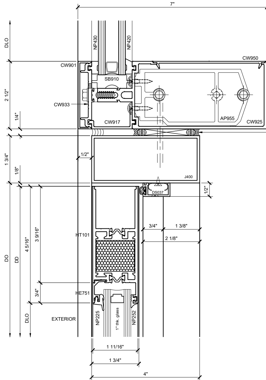
SECTION DETAIL @ DOOR HEAD w/ OHCC 18 SCALE: FULL SIZE
