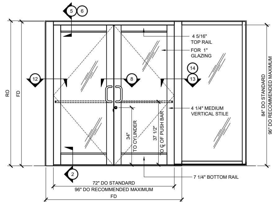
MEDIUM STILE SERIES 400AT DOOR TYP. ELEVATION (DOUBLE DOOR @ UP / OVER FRAME WITH SIDELITE) 3/4" =1'-0"
