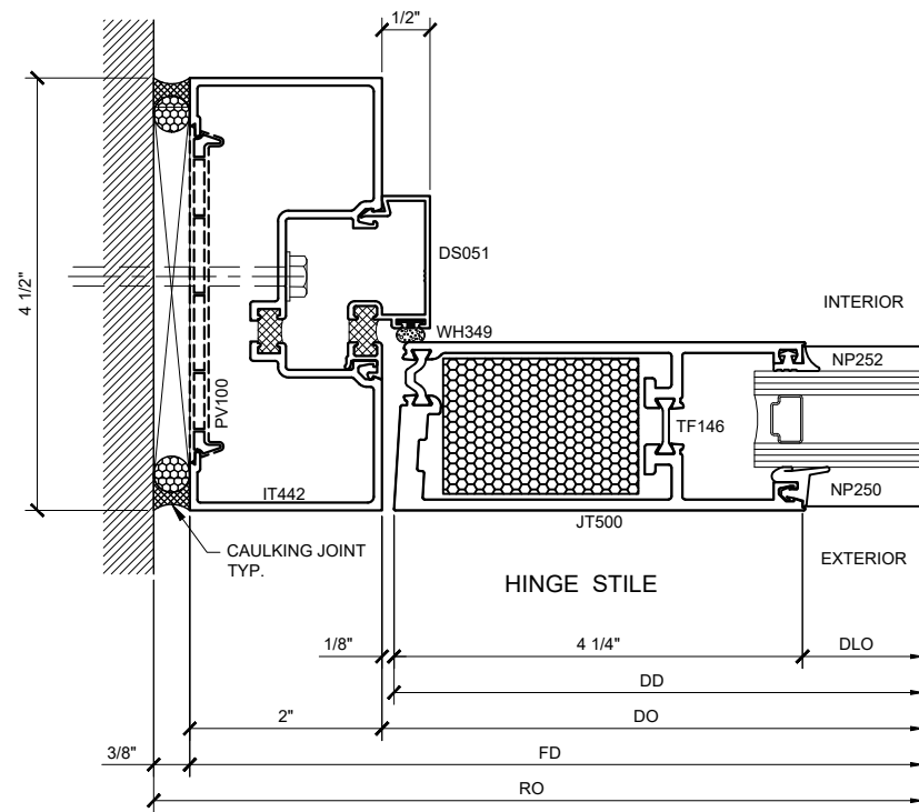
SECTION DETAIL @ DOOR JAMB 10 SCALE: FULL SIZE
