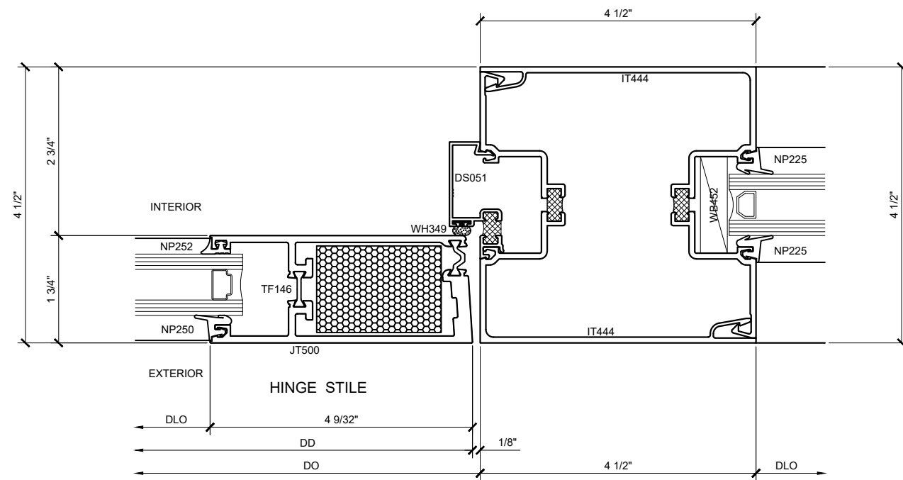
SECTION DETAIL AT WIDE HINGE STYLE INTERMEDIATE VERTICAL (14) SCALE: FULL SIZE
