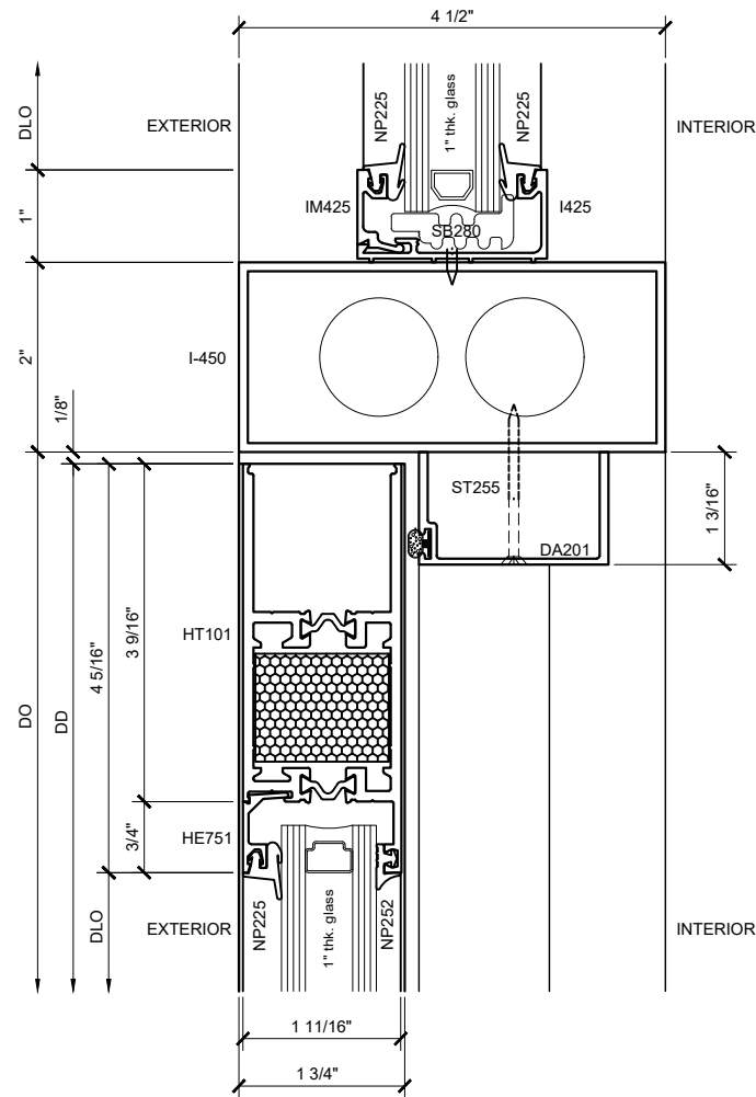
SECTION DETAIL @ DOOR HEAD w/ OHCC ③ SCALE: FULL SIZE
