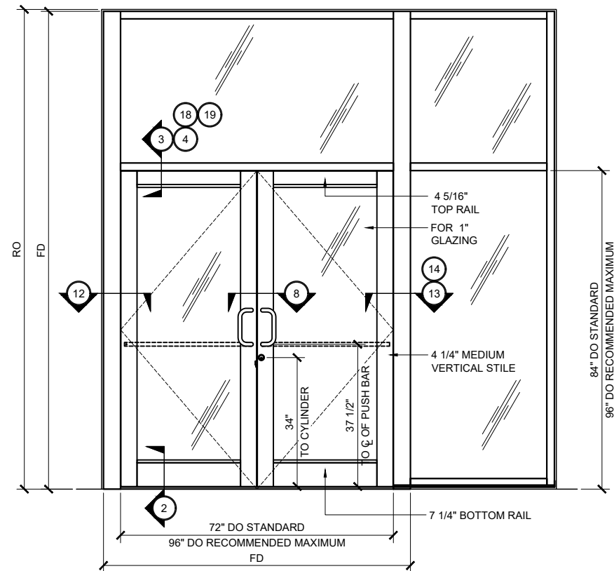
MEDIUM STILE SERIES 400AT DOOR TYP. ELEVATION (DOUBLE DOOR @ TRANSOM FRAME ) 3/4" =1'-0"
