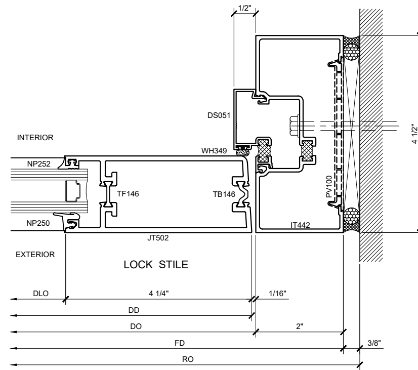
SECTION DETAIL @ DOOR JAMB 11 SCALE: FULL SIZE
