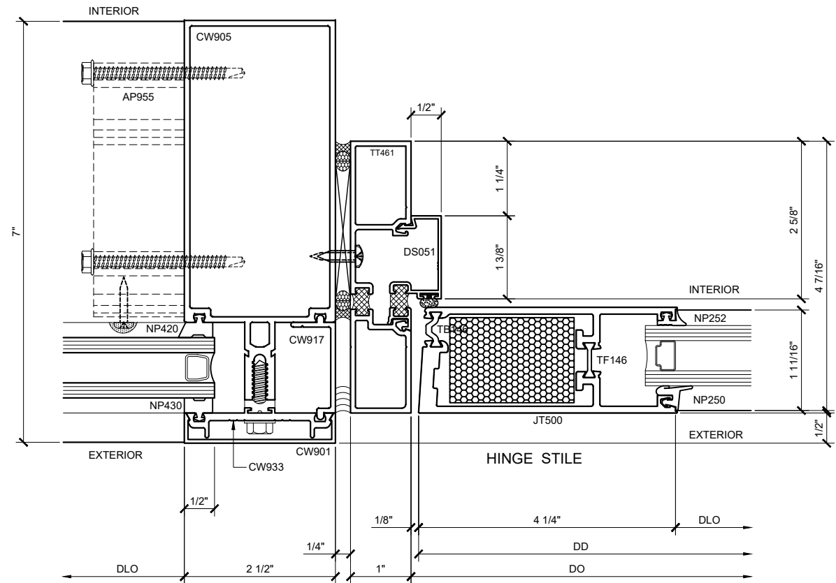
SECTION DETAIL @ DOOR JAMB (20) SCALE: FULL SIZE
