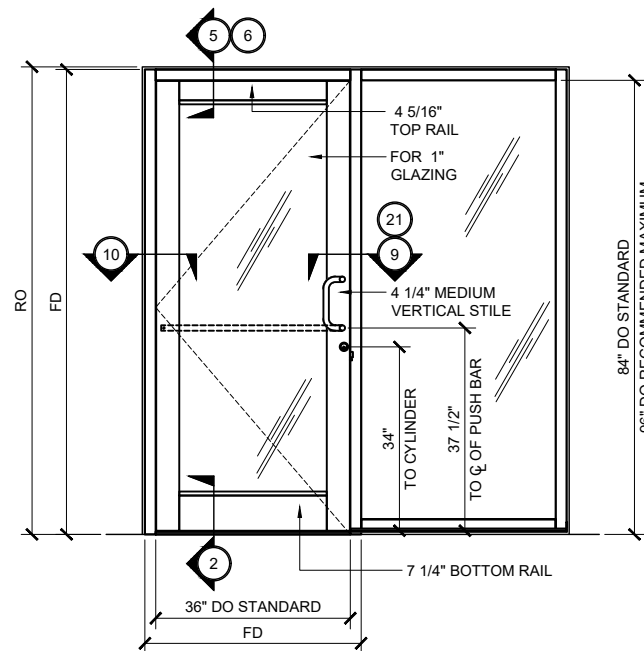
MEDIUM STILE SERIES 400AT DOOR TYP. ELEVATION (SINGLE DOOR @ UP / OVER FRAME WITH SIDELITE) 3/4" = 1'-0"
