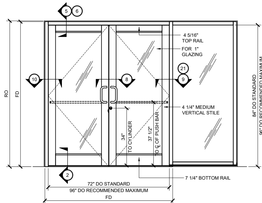
MEDIUM STILE SERIES 400AT DOOR TYP. ELEVATION (DOUBLE DOOR @ UP / OVER FRAME WITH SIDELITE) 3/4" = 1'-0"
