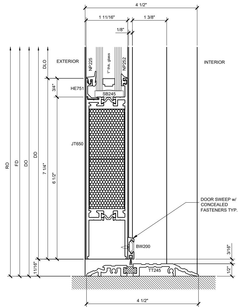
SECTION DETAIL @ 7 1/4" DOOR SILL ②
