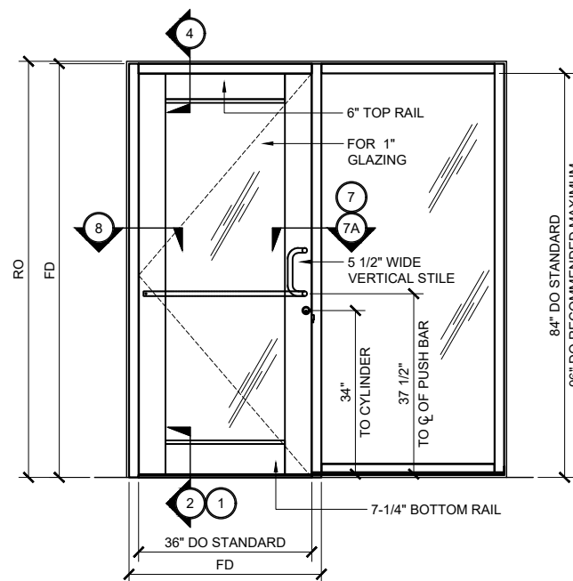
WIDE STILE SERIES 550T DOOR TYP. ELEVATION (SINGLE DOOR @ UP / OVER FRAME WITH SIDELITE) 3/4" = 1'-0"
