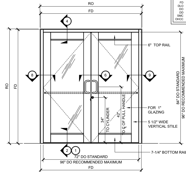
WIDE STILE SERIES 550T DOOR TYP. ELEVATION (DOUBLE DOOR @ UP / OVER FRAME) 3/4" = 1'-0"
