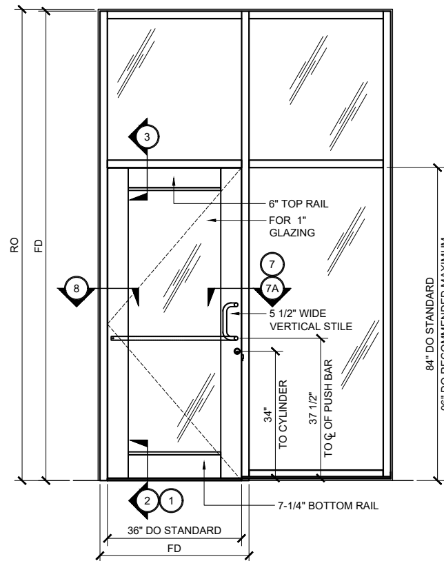
WIDE STILE SERIES 550T DOOR TYP. ELEVATION (SINGLE DOOR @ TRANSOM FRAME) 3/4" = 1'-0"
