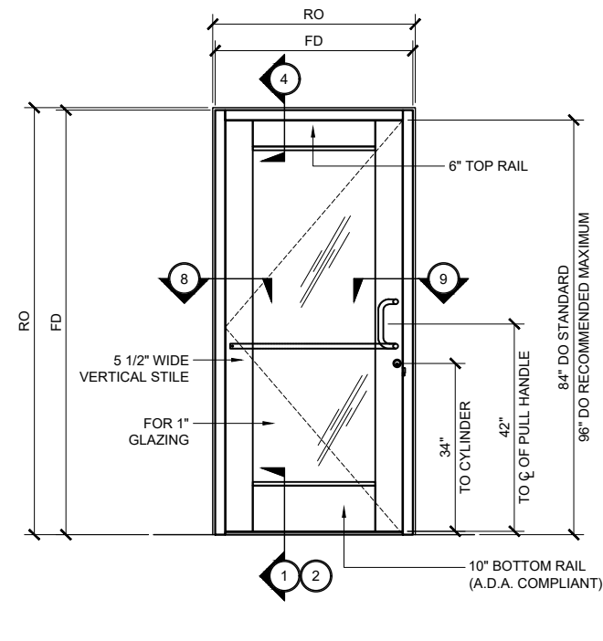
WIDE STILE SERIES 550T DOOR TYP. ELEVATION (SINGLE DOOR @ UP / OVER FRAME) (SHOWN W/ 10" COMPLIANT BOTTOM RAIL) 3/4" = 1'-0"
