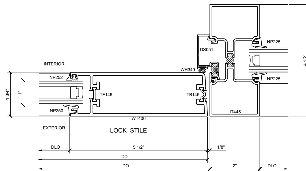
SECTION DETAIL @ DOOR JAMB (7A) SCALE: FULL SIZE
