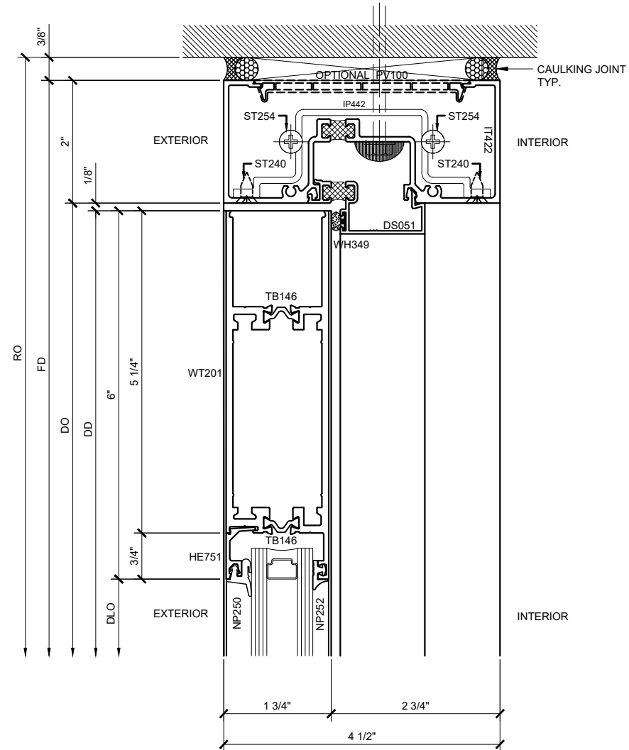
SECTION DETAIL @ DOOR HEAD (4) SCALE: FULL SIZE
