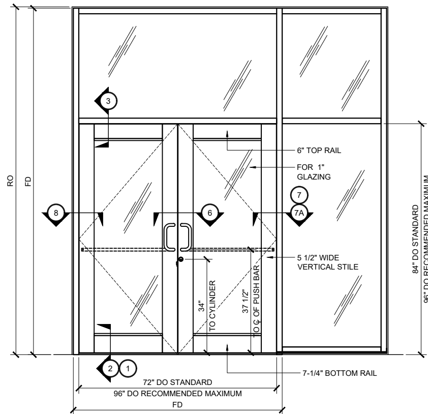
WIDE STILE SERIES 550T DOOR TYP. ELEVATION (DOUBLE DOOR @ TRANSOM FRAME) 3/4" = 1'-0"
