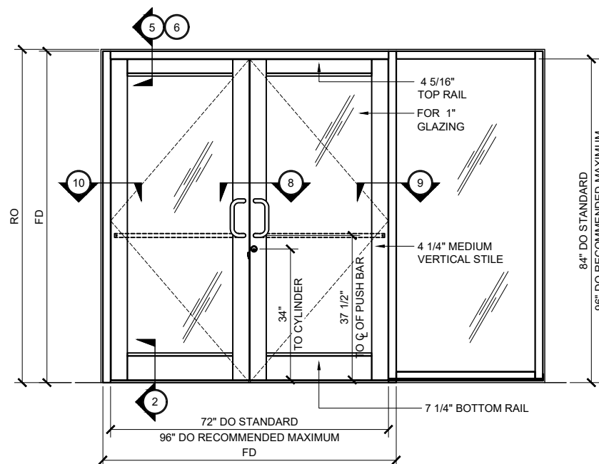
MEDIUM STILE SERIES 400T DOOR TYP. ELEVATION (DOUBLE DOOR @ UP / OVER FRAME WITH SIDELITE) 3/4" = 1'-0"
