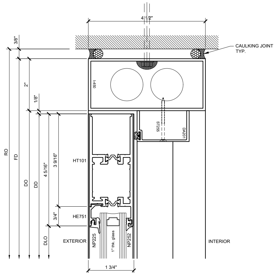
SECTION DETAIL @ DOOR HEAD w/ OHCC (5) SCALE: FULL SIZE
