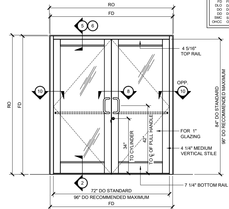
MEDIUM STILE SERIES 400T DOOR TYP. ELEVATION (DOUBLE DOOR @ UP / OVER FRAME) 3/4" = 1'-0"
