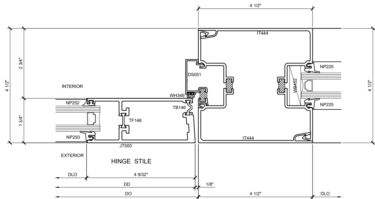
SECTION DETAIL AT WIDE HINGE STYLE INTERMEDIATE VERTICAL (17) SCALE: FULL SIZE
