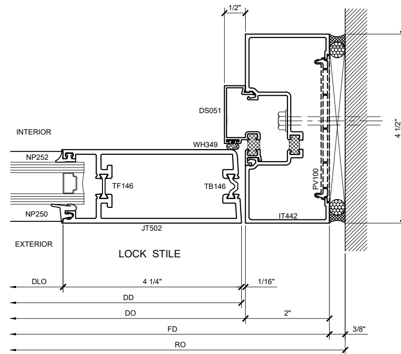
SECTION DETAIL @ DOOR JAMB 11
