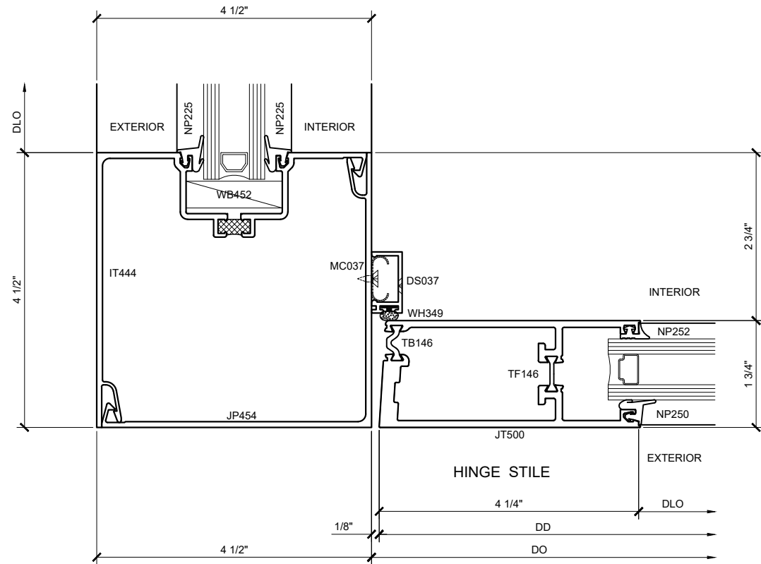
SECTION DETAIL AT WIDE HINGE STYLE CORNER VERTICAL (15) SCALE: FULL SIZE
