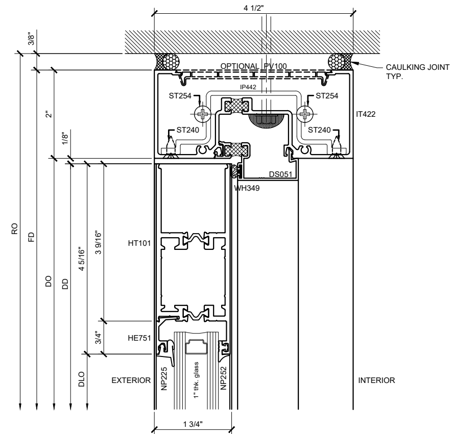
SECTION DETAIL @ DOOR HEAD (6) SCALE: FULL SIZE
