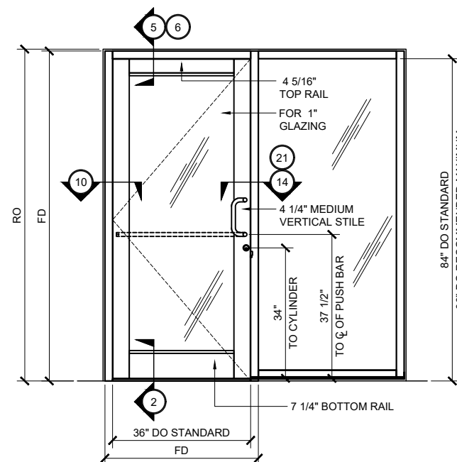
MEDIUM STILE SERIES 400T DOOR TYP. ELEVATION (SINGLE DOOR @ UP / OVER FRAME WITH SIDELITE) 3/4" = 1'-0"
