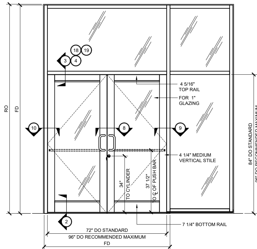
MEDIUM STILE SERIES 400T DOOR TYP. ELEVATION (DOUBLE DOOR @ TRANSOM FRAME) 3/4" = 1'-0"
