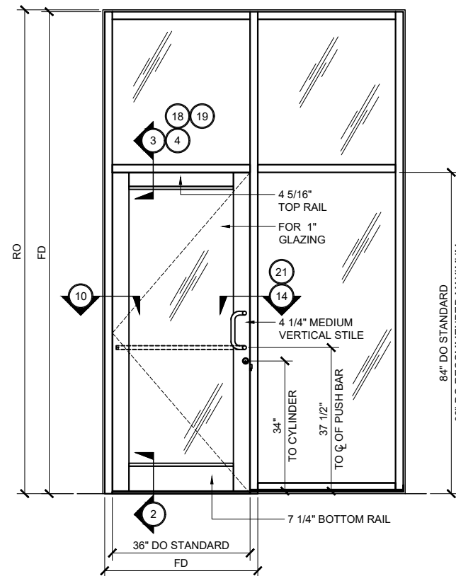
MEDIUM STILE SERIES 400T DOOR TYP. ELEVATION (SINGLE DOOR @ TRANSOM FRAME) 3/4" = 1'-0"
