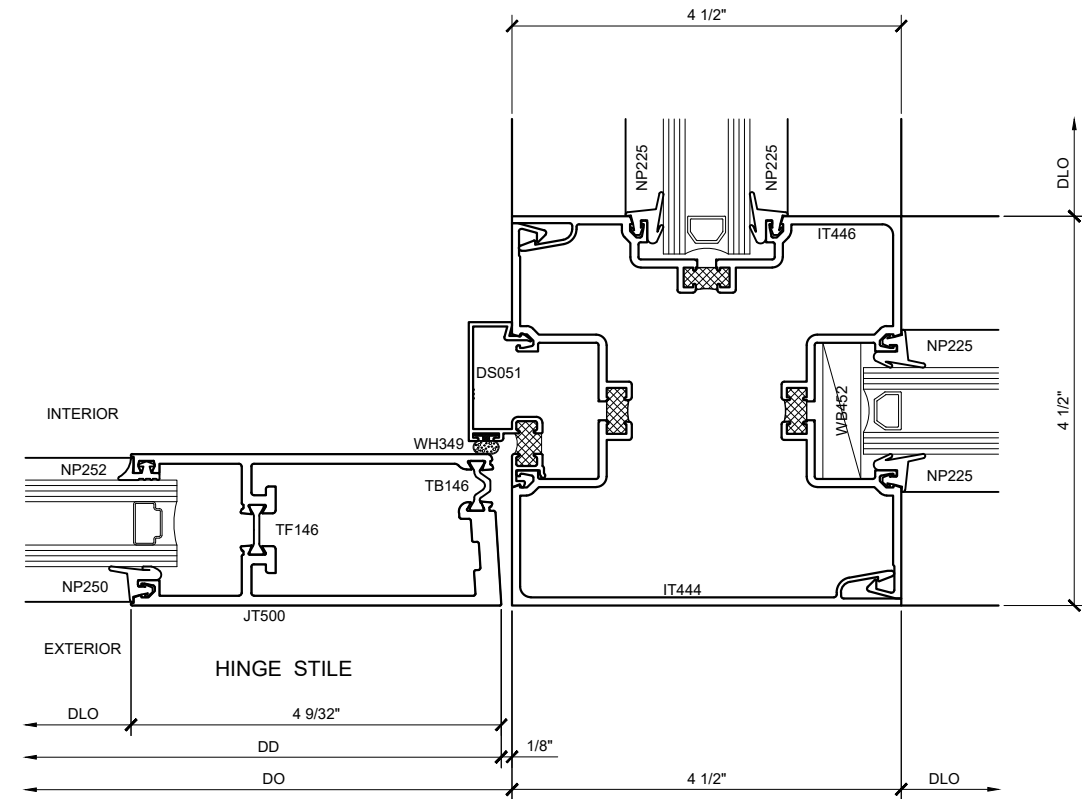
SECTION DETAIL AT WIDE HINGE STYLE "T" VERTICAL (16) SCALE: FULL SIZE
