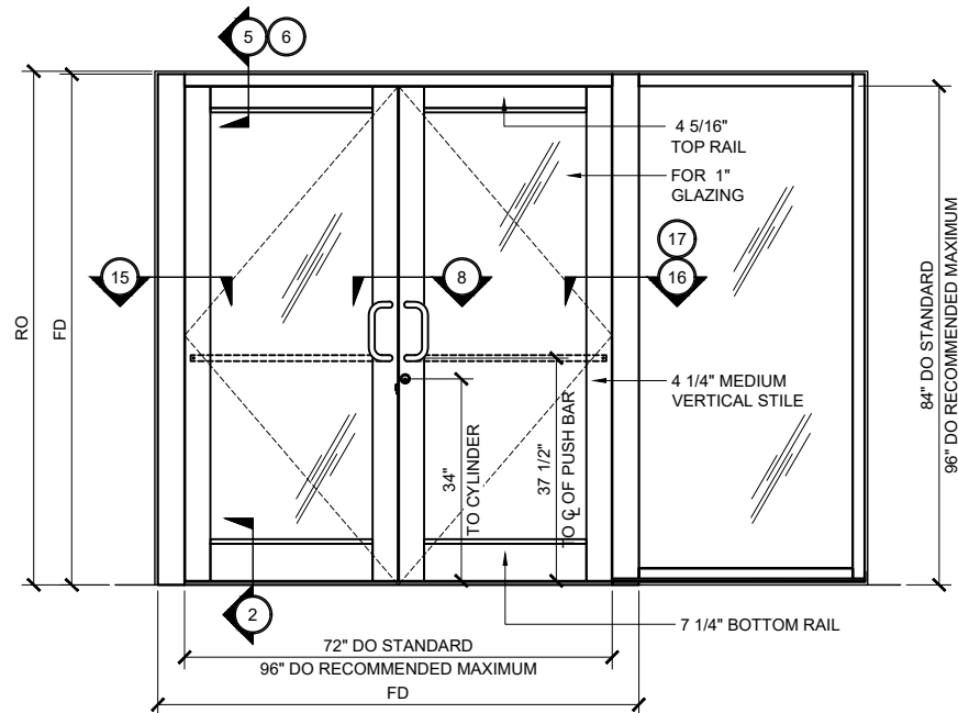
MEDIUM STILE SERIES 400T DOOR TYP. ELEVATION (DOUBLE DOOR @ UP / OVER FRAME WITH SIDELITE) 3/4" = 1'-0"
