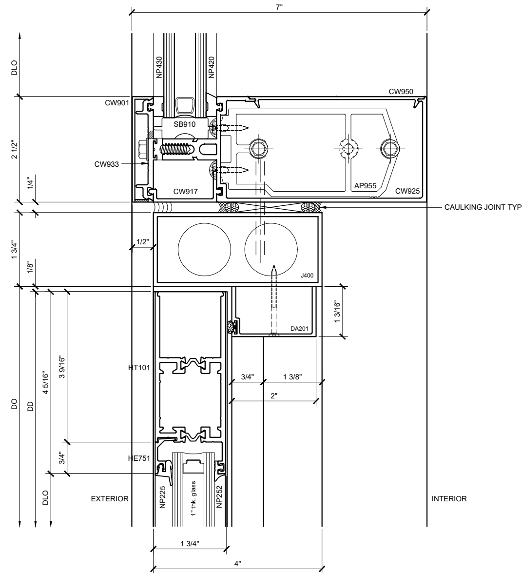
SECTION DETAIL @ DOOR HEAD w/ OHCC 19 SCALE: FULL SIZE
