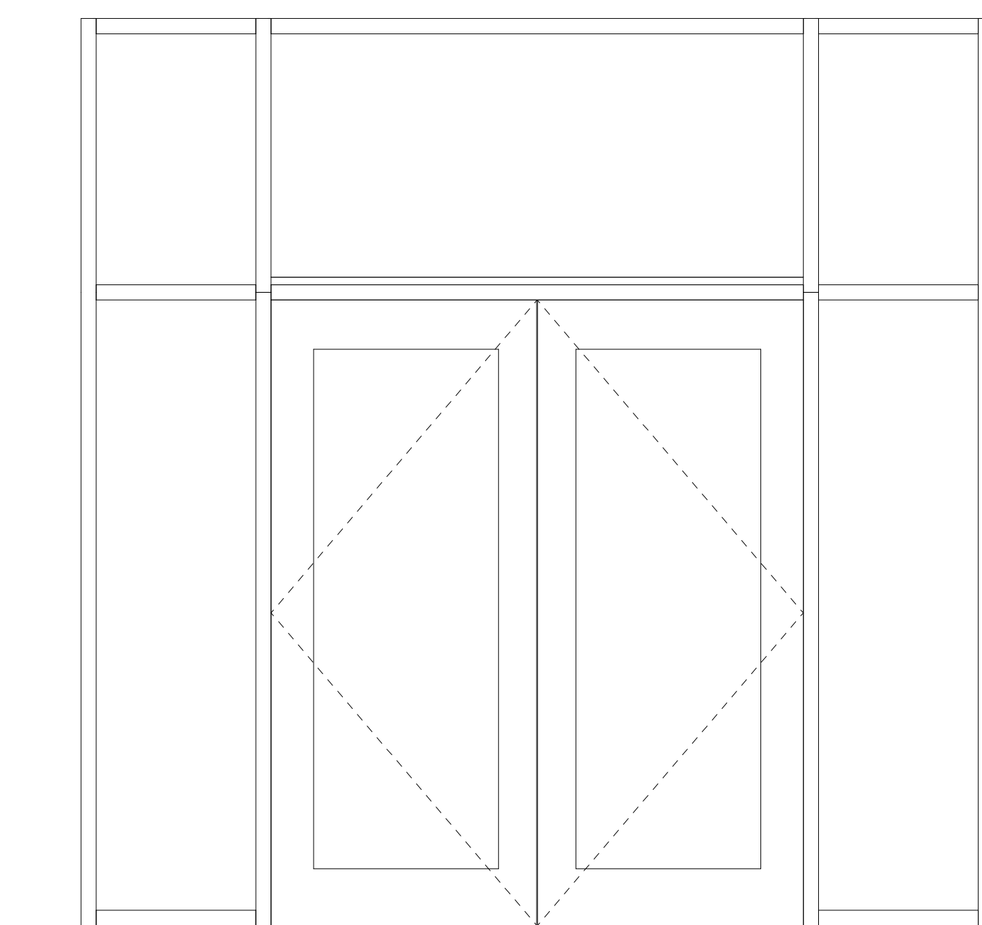
⑨ 250 - 400 - 550 Double Elevation 3/4" = 1'-0"
