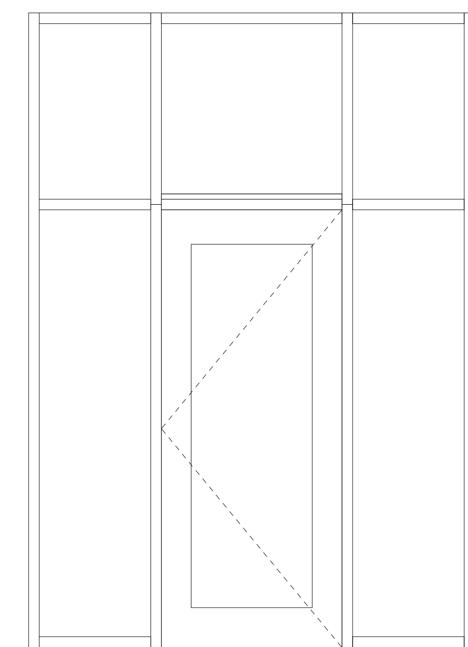
② 250 - 400 - 550 Single Elevation 3/4" = 1'-0"
