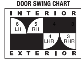
Use the Door Swing Chart to determine how the door(s) should be handed.
